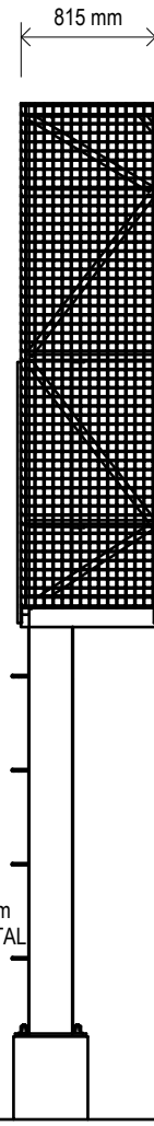
SIDE ELEVATION
