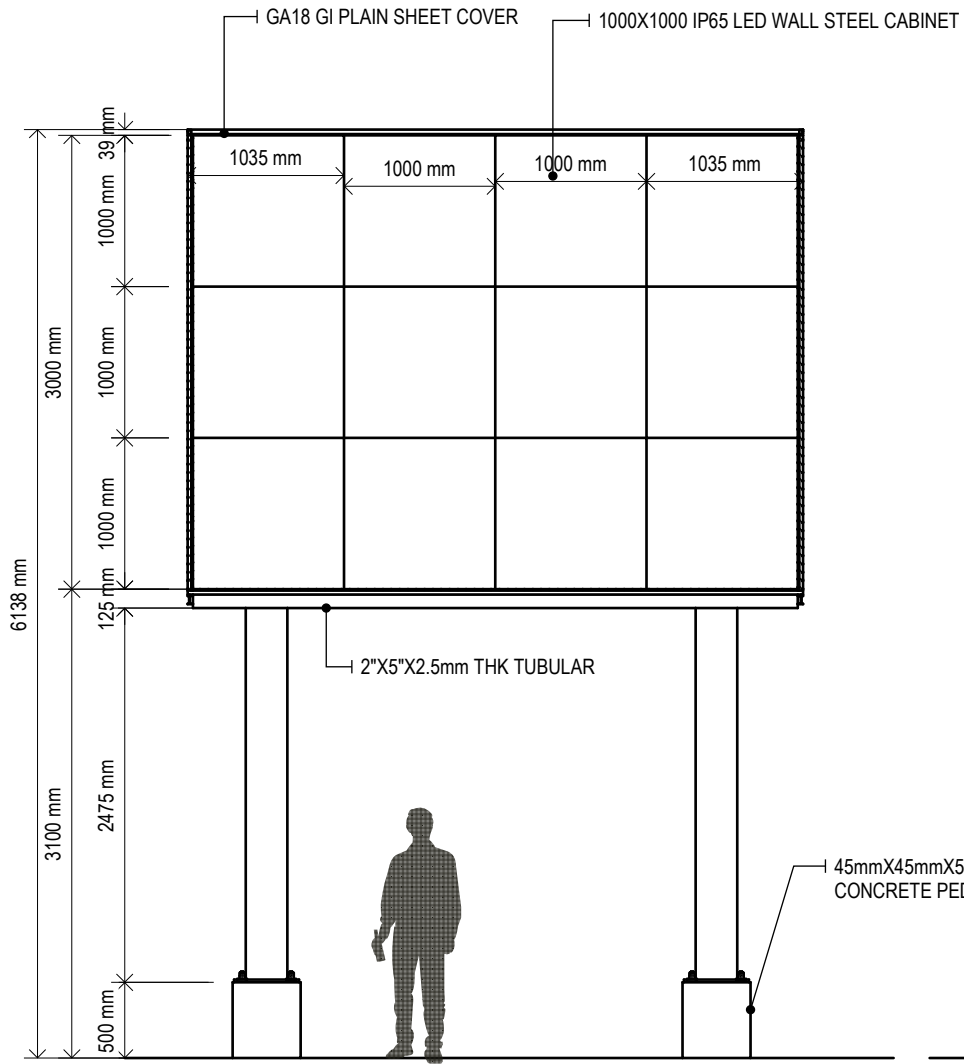
FRONT ELEVATION
