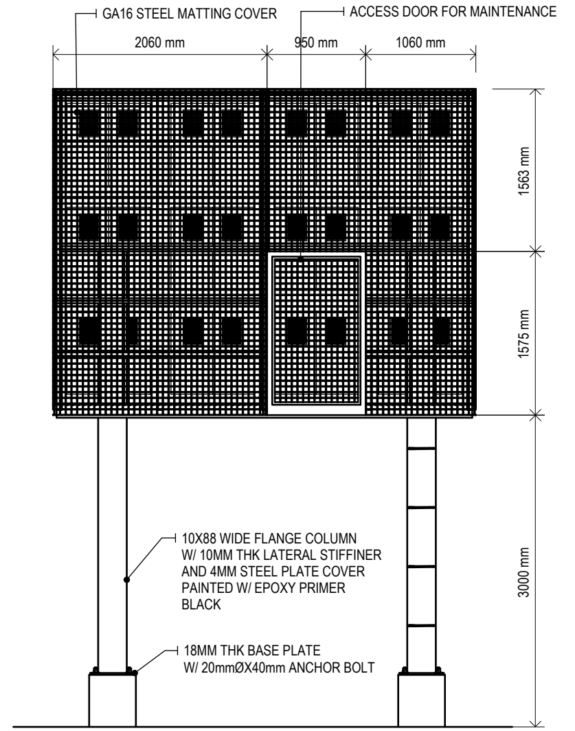
REAR ELEVATION
